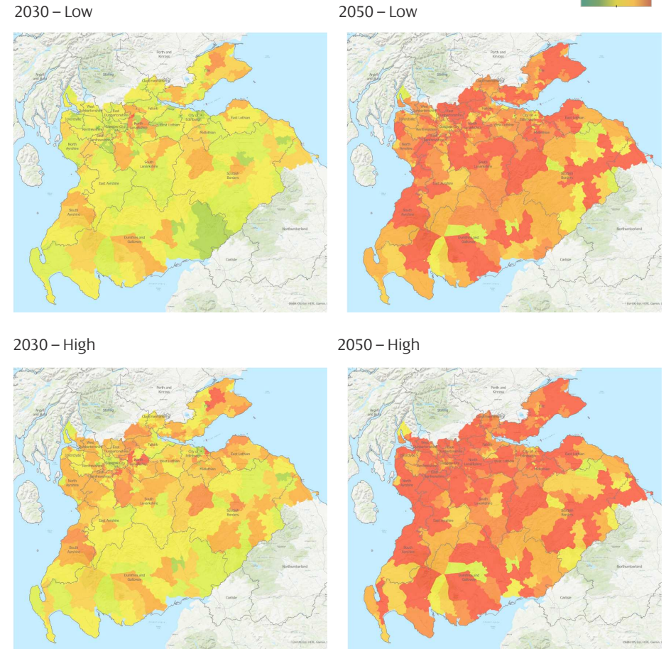
Figure 3 | Electricity peak demand changes from 2020 by primary substation area. Scale range: -2MW to >10MW
