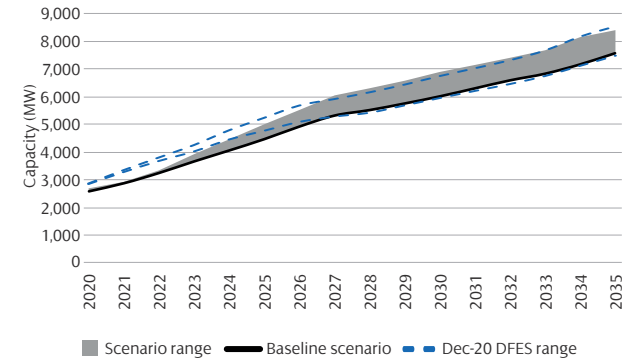
Figure 12 | Range of Net Zero compliant distributed generation forecasts
