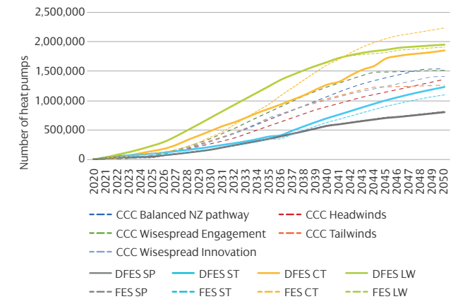
Figure 10 | Heat pump uptake comparison
